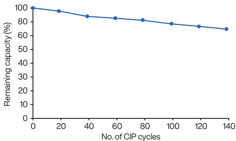
Figure 3. DBC for HlgG on WorkBeads affimAb Edge determined by frontal analysis at 4 minutes residence time after 140 CIP cycles with 0.5 M NaOH at 15 minutes contact time.
