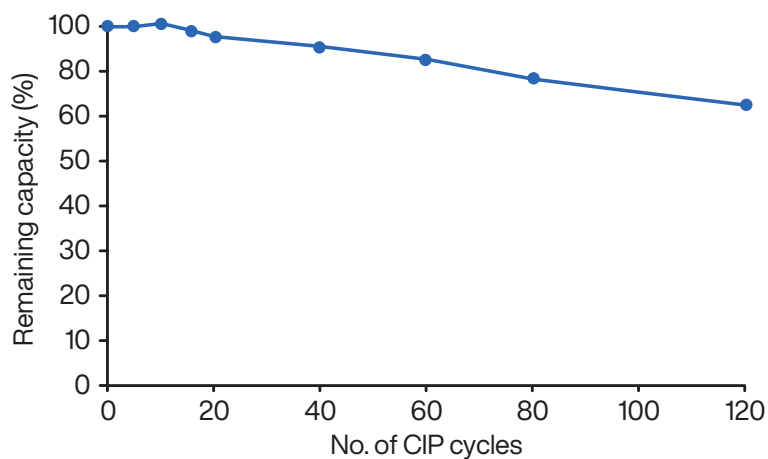
Figure 2. DBC for polyclonal human IgG on WorkBeads affimAb determined by frontal analysis at 2.5 minutes residence time after 120 CIP cycles using 0.5 M NaOH at 15 minutes contact time.
