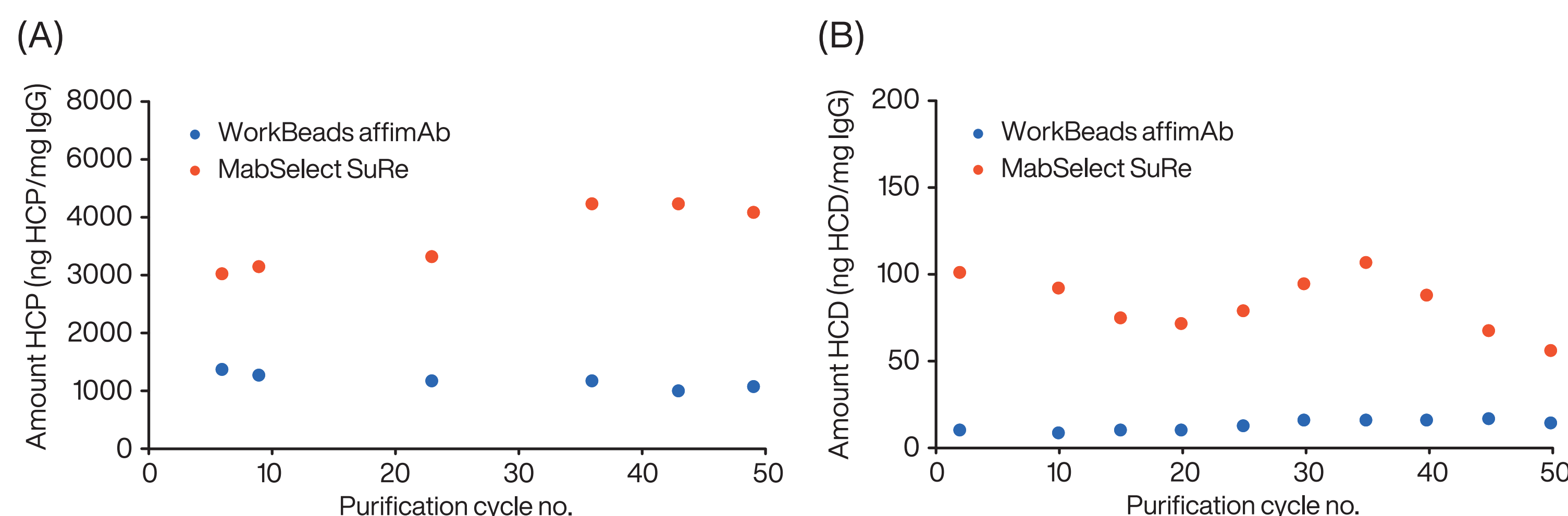
Figure 3. Comparison of residual HCP (A) and HCD (B) in mAb eluates from WorkBeads affimAb and MabSelect SuRe during 50 purification cycles.
