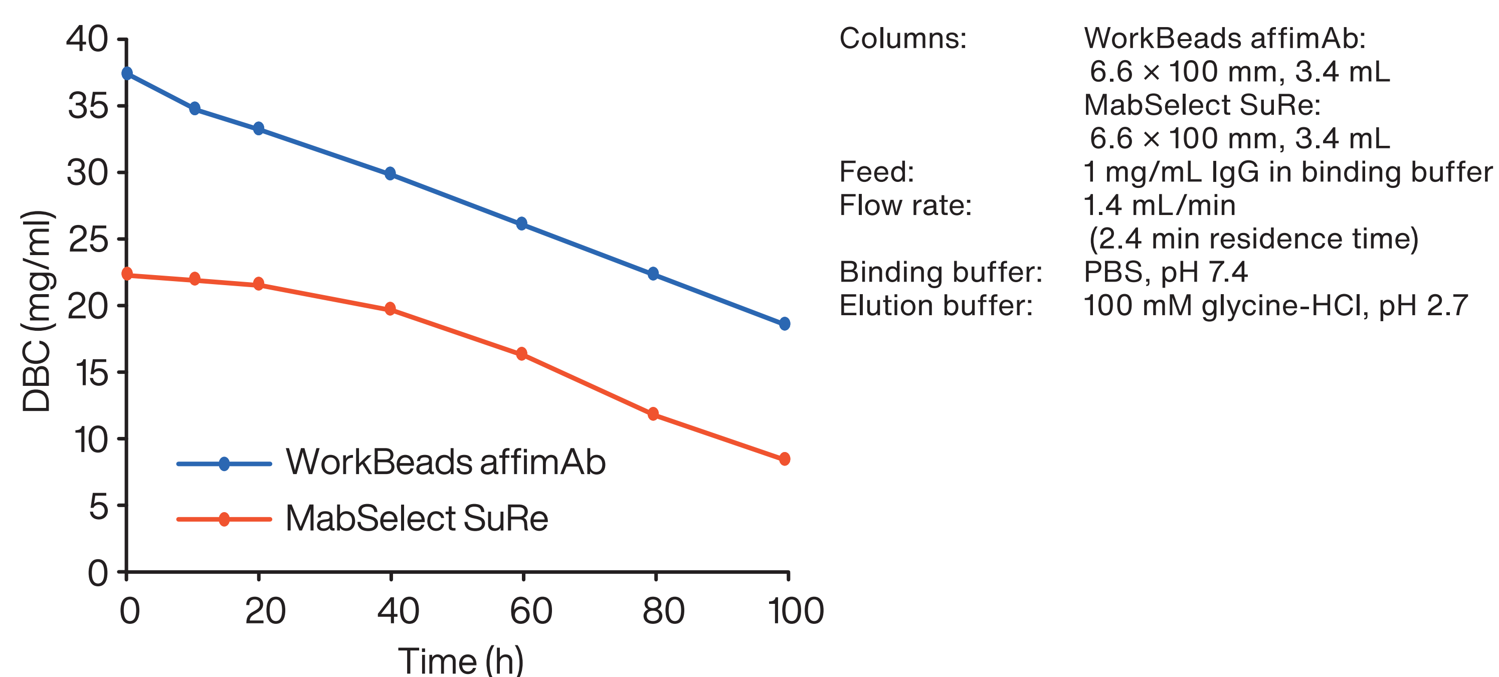
Figure 2. DBC determined with polyclonal human IgG at 2.4 min residence time. Q_{B10\%} measured at every 20 th CIP cycle for WorkBeads affimAb and MabSelect SuRe.
