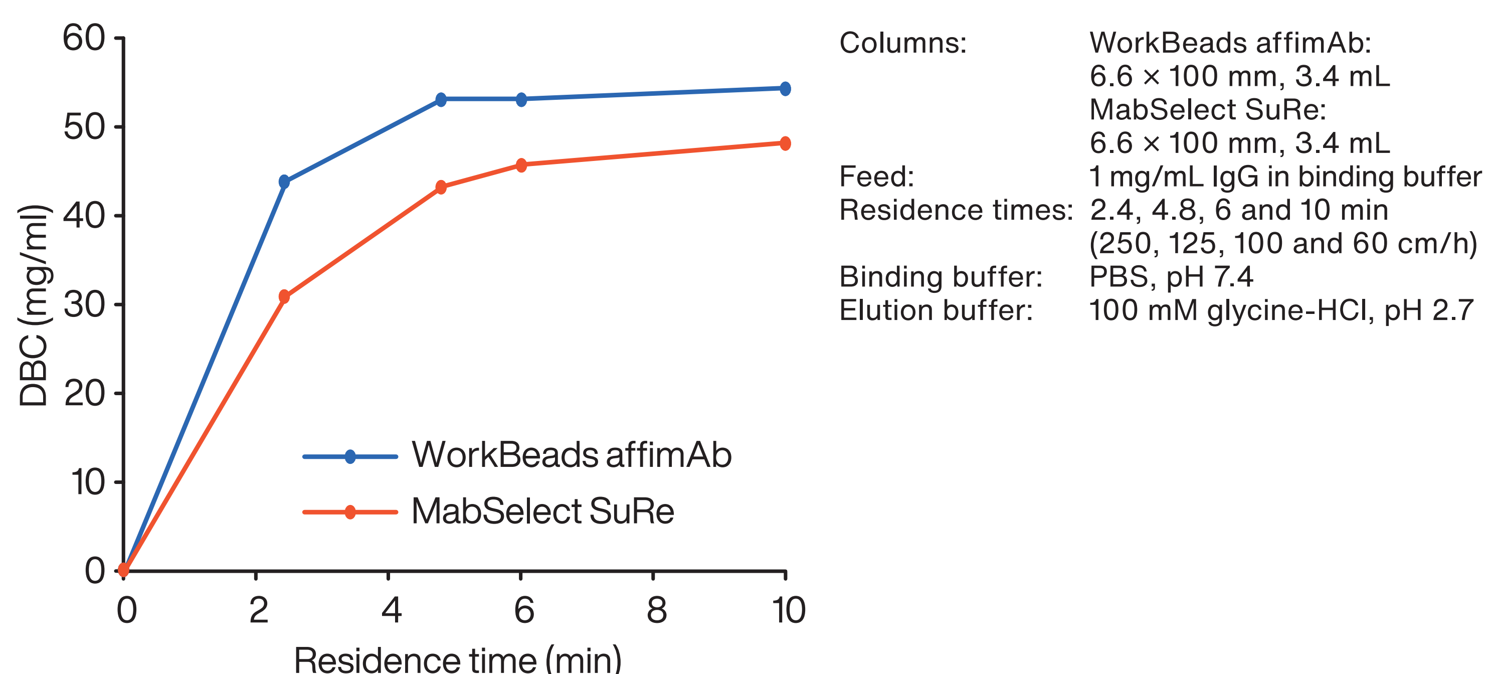
Figure 1. DBC for human polyclonal IgG determined at different flow rates (residence times) by frontal analysis on WorkBeads affimAb (blue) and MabSelect SuRe (red).
