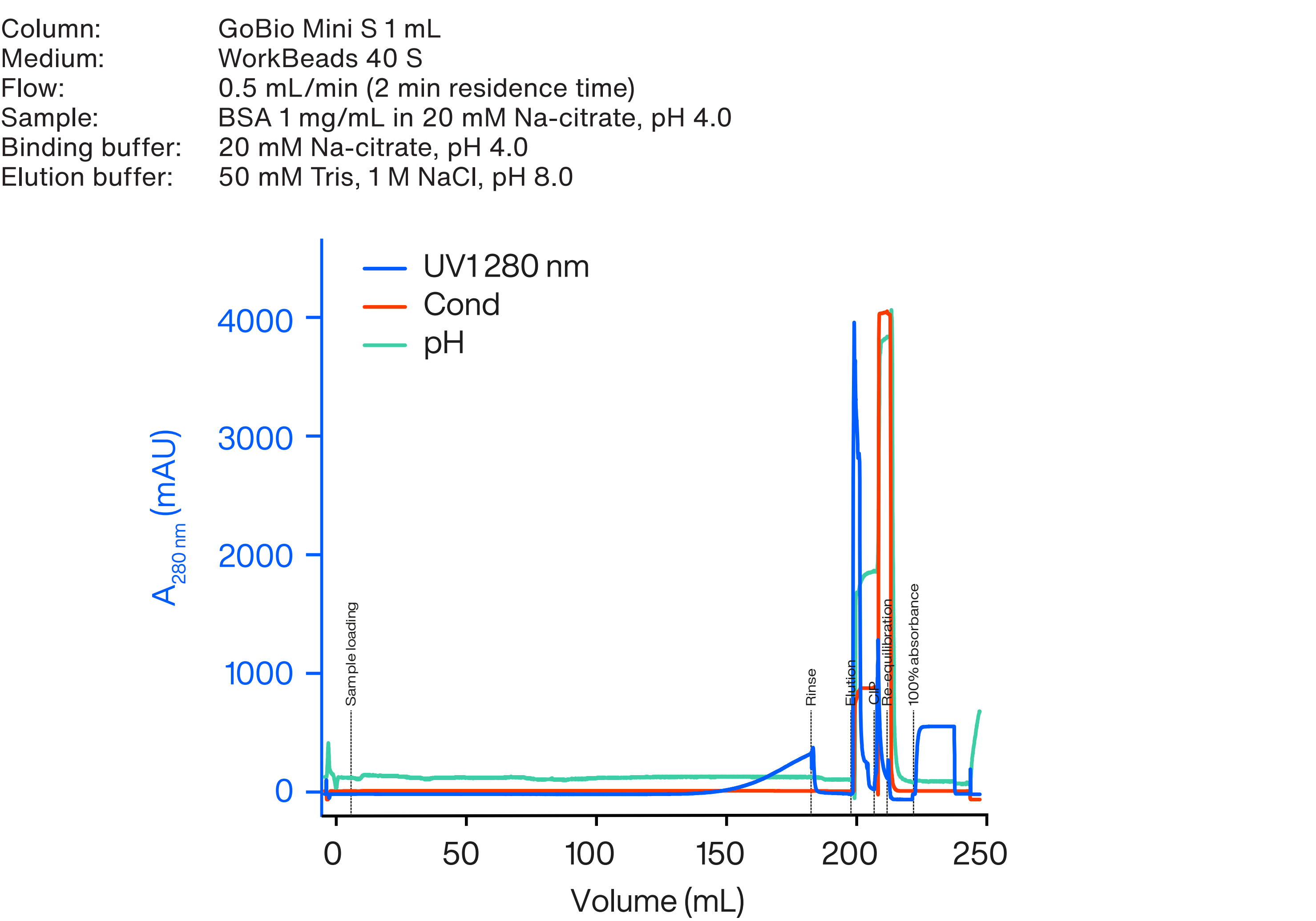
Figure 2. Example of chromatogram from experiment N2 on GoBio™ Mini S 1 mL column. The DBC for these conditions was 145 mg/mL.
