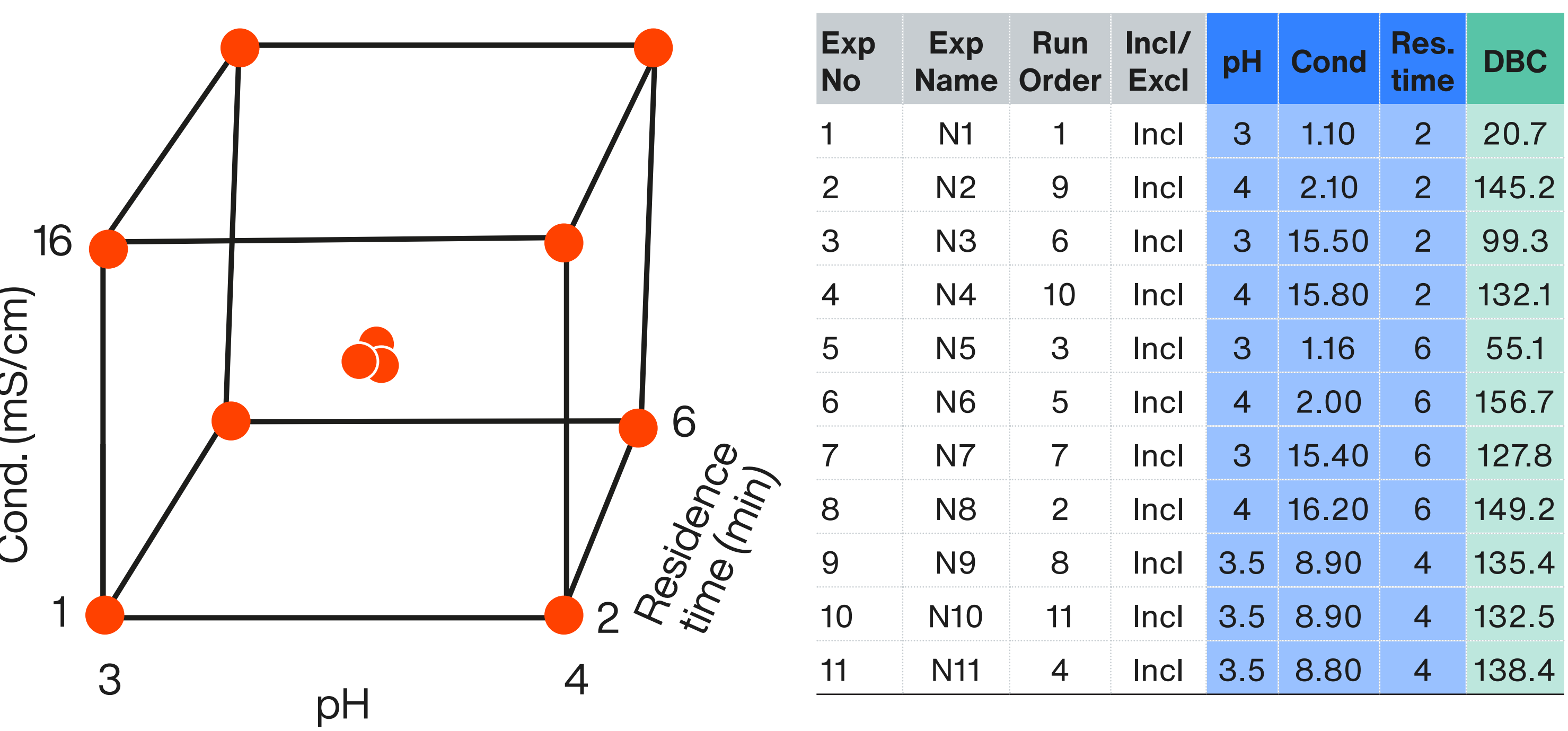
Figure 1. The design region. The ranges were for pH was 3–4, conductivity 1–16 mS/cm (corresponding to 0–120 mM NaCl), and residence times 2–6 minutes.
