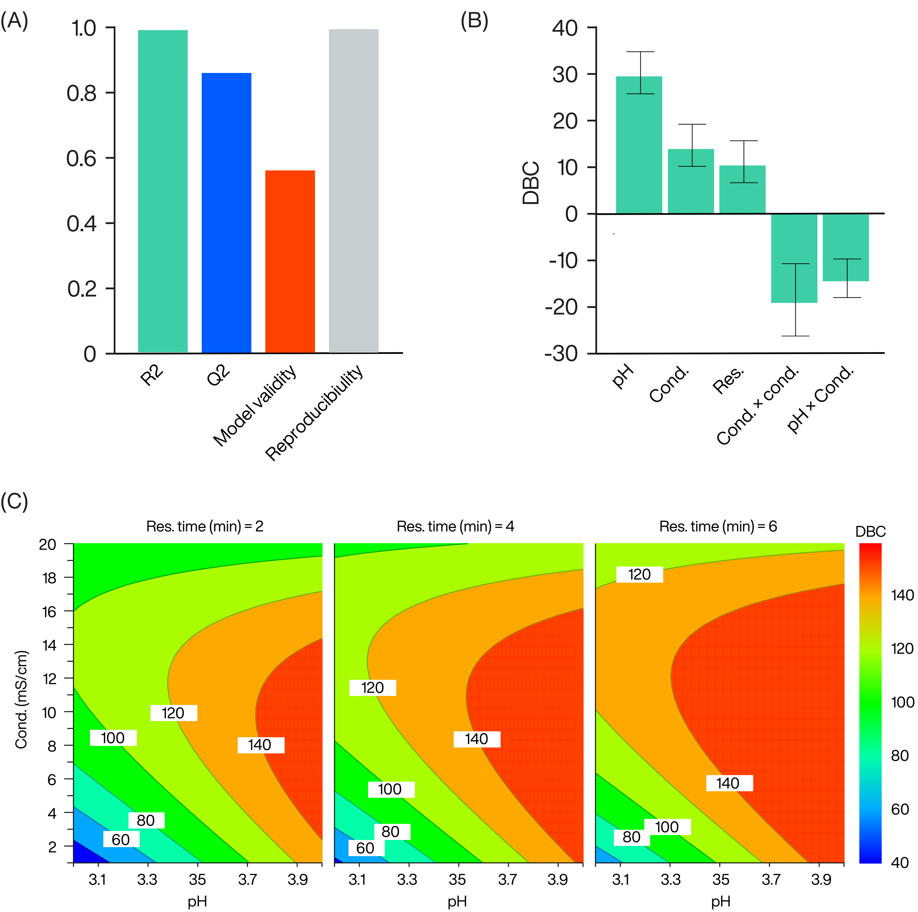
Figure 3. Evaluation of the study.
